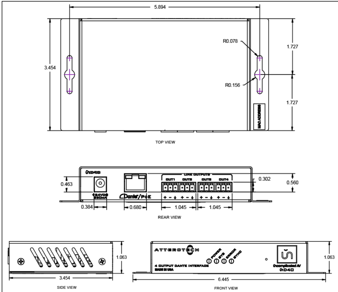
Figure 2 - Mounting Information
